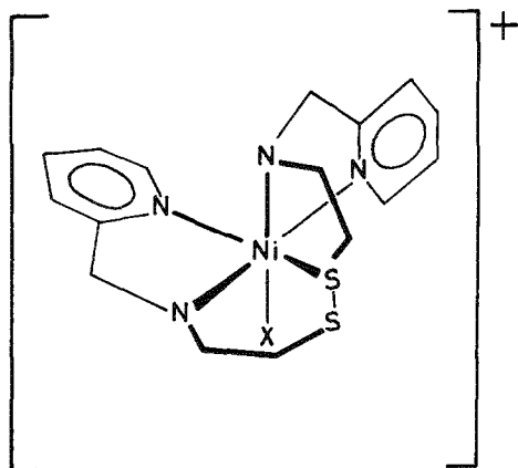
VIII (X = Cl)
